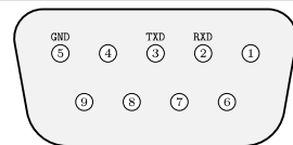
SubD-9 female
