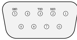
SubD-9 female
